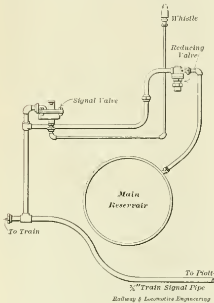
FIG. 3.—SIGNAL PIPING.
